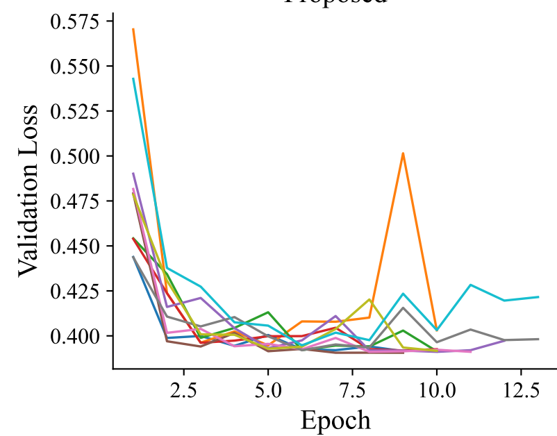
Proposed
