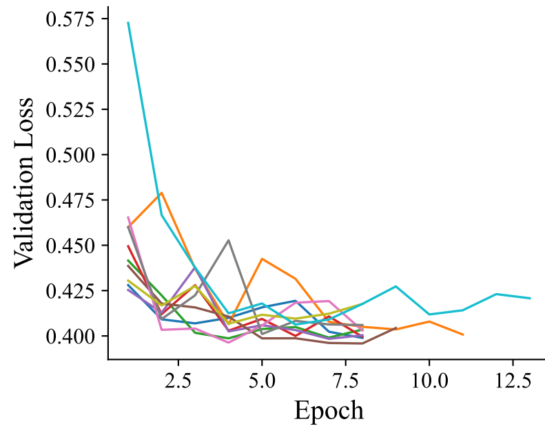
ResNet18
