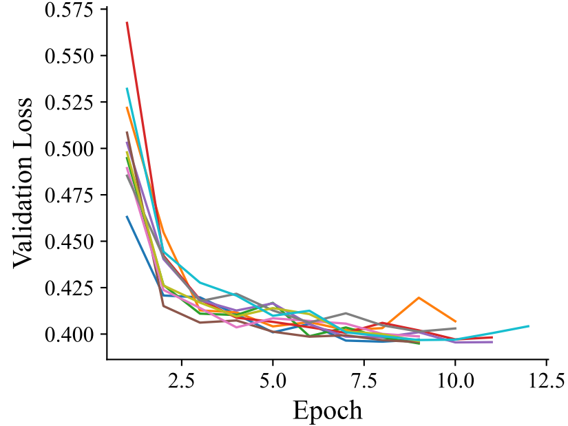
MobileNetV3-Small
