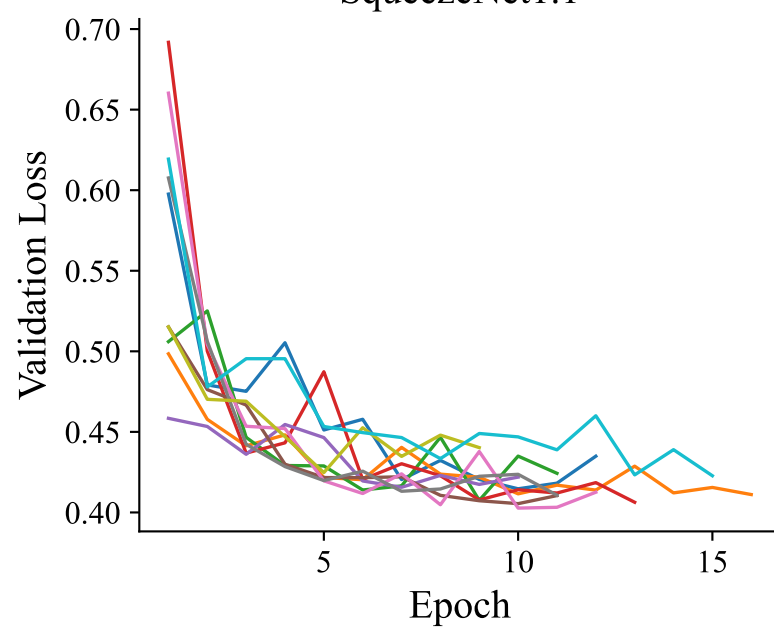
SqueezeNet1.1
